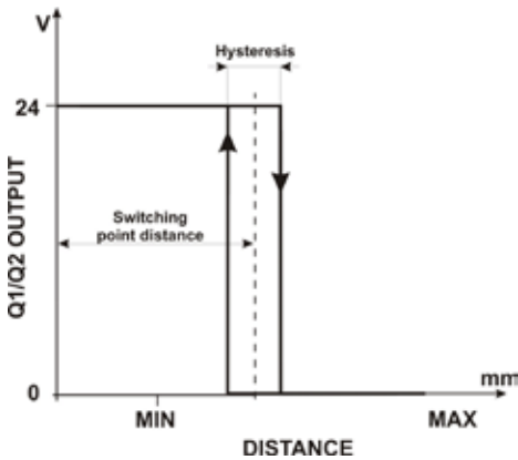
HYSTERESIS
